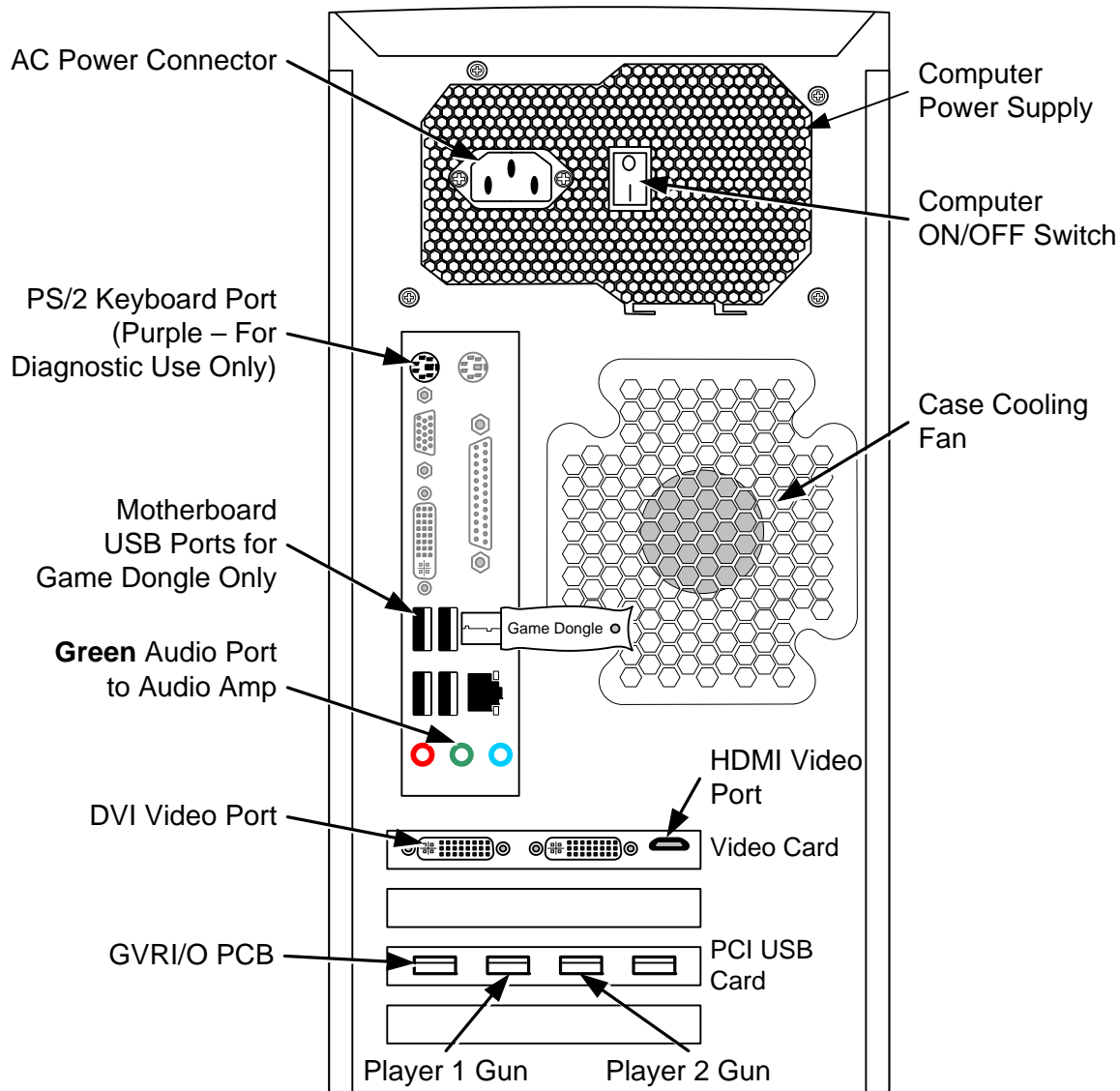
Figure 1. Computer Rear Panel Diagram (DG41TX Motherboard)
