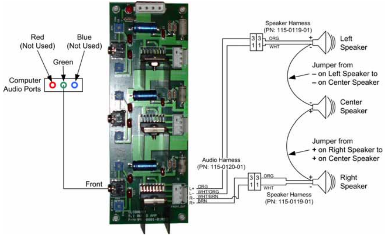
Figure 5. Adding Jumpers for Center Speaker Audio with 5.1 Audio Amp
