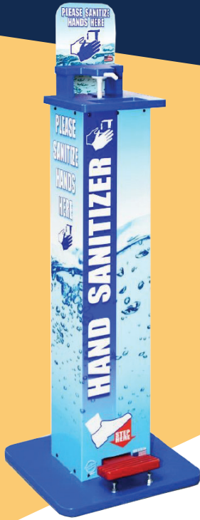
STANDARD MODEL
