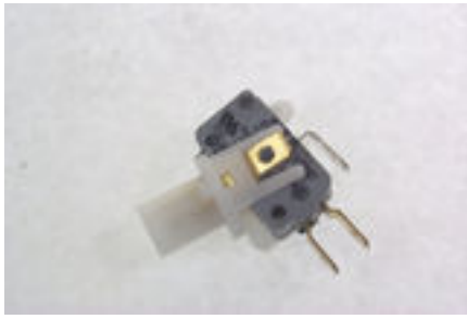
2150.0120 Bulbholder & microswitch for pushbutton
