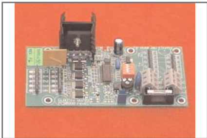
9002.0982 Pcb chaserlight low voltage
