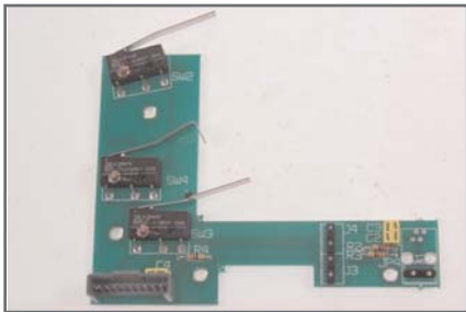
9002.0031 Pc board grab-stop Eurograb
